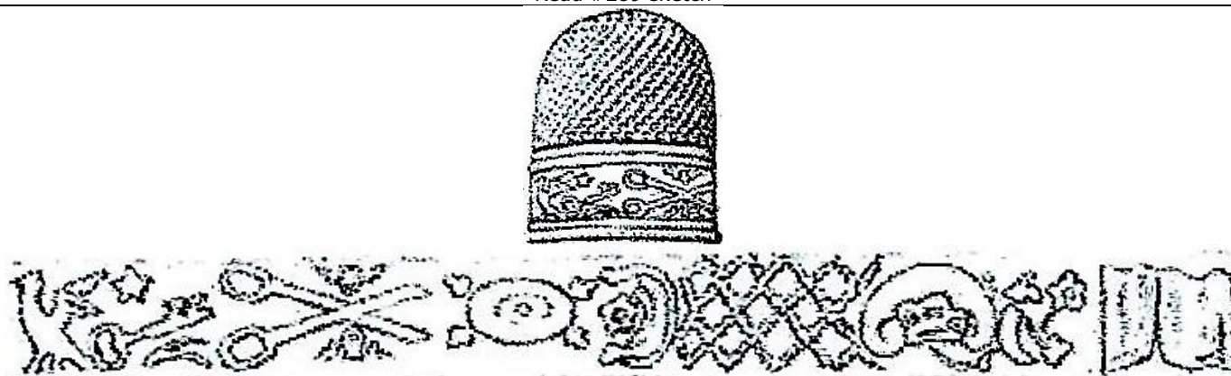
Read #290 sketches
